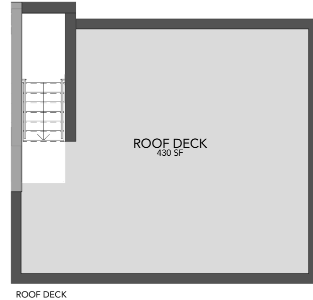
ROOF DECK
